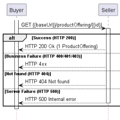
Figure 19. Use Case 4 - Retrieve Product Offering by Identifier
